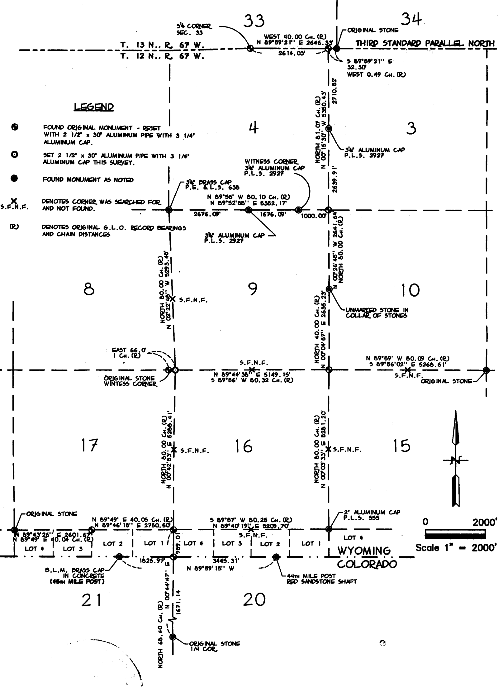
SKETCH OF SURVEY T. 12 N., R. 67 W., 6TH P.M. LARAMIE COUNTY, WYOMING
